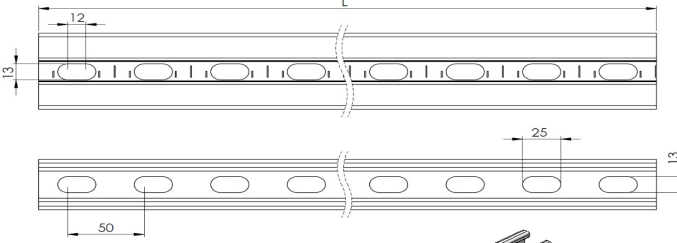
41X62 C PROFILE
